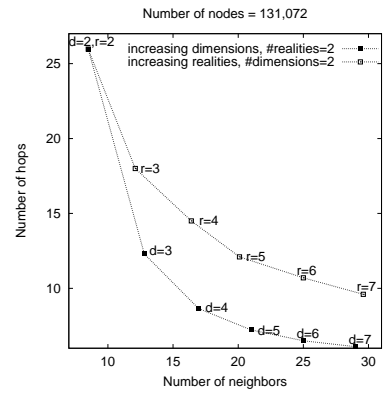
Figure 6: Path length with increasing neighbor state
