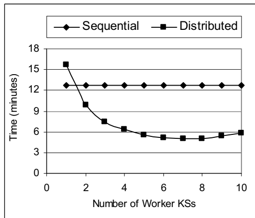
Fig 12 Sequential and distributed NC similarity metric performance with increasing numbers of Worker agents.
