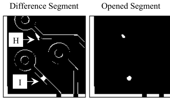
Fig 10 Referential comparison of the fixed and registered segments reveals printed circuit board defects.
