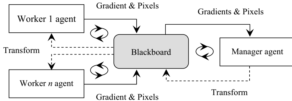
Fig 7 Flow of gradient data and updated transform parameters between agents.
