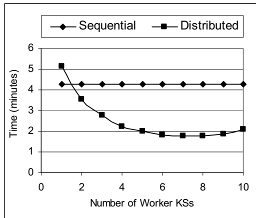
Fig 11 Sequential and distributed MS similarity metric performance with increasing numbers of Worker agents.
