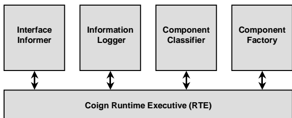
Figure 2. Coign Runtime Architecture.
