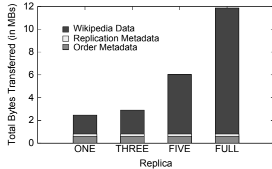
Figure 12: Bandwidth consumption for transferring data, order metadata, and replication metadata to replicas with different content adaptation levels.
