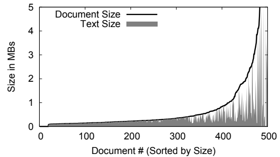
Figure 6: The distribution of the size of text content in a Word 2007 (docx) document compared to its total size.
