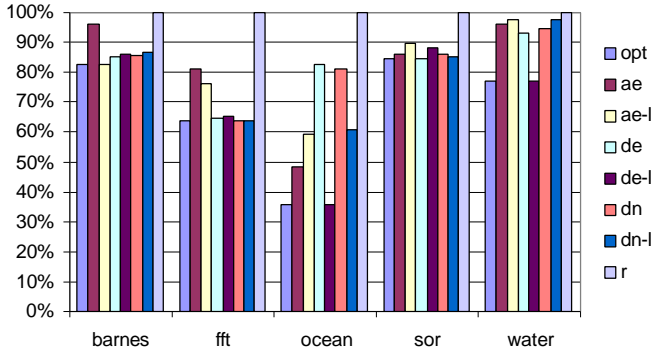
Figure 6: Normalized 8-processor execution times
