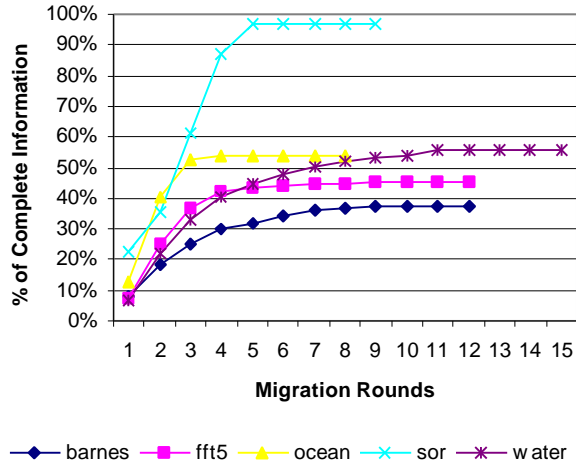
Figure 3: Passive Information-Gathering
