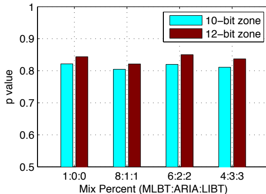
Fig. 5: 10-bit and 12-bit zone’s p value as a function of different mix percents of three applications. stdev is small therefore omitted from the figure. 10-bit zone’s stdev is consistently smaller than 12-bit zone’s. (MLBT: Mainline BitTorrent; ARIA: Aria; LIBT: libtorrent)
