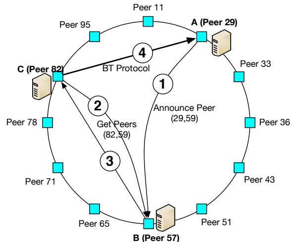
Fig. 1: Normal operation of MLDHT
