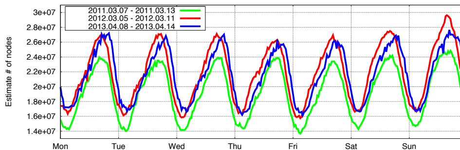
Fig. 7: One week 2011, 2012, and 2013. The weeks show the typical daily churn, mainly caused by East European users. The typical number of users increased by about 10% from 2011 to 2012, but has remained stable since then.
