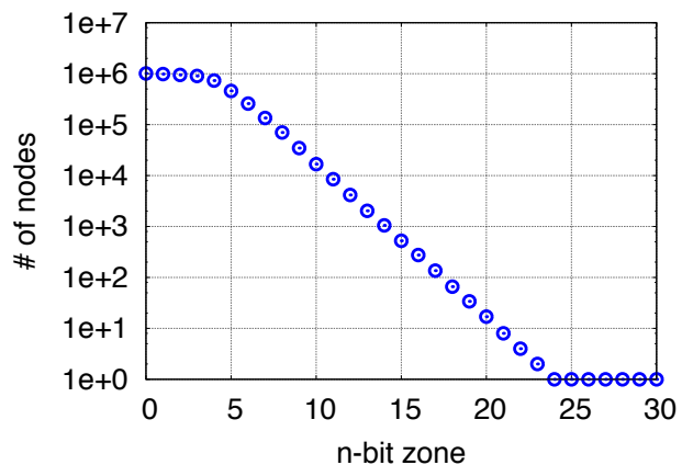
Fig. 2: Number of nodes discovered by our crawler in different n -bit zones. There were about 20 million nodes in the system when the experiment was performed. With 5-bit zone, the crawler reached its performance limit and many nodes were missed. Beyond a 24-bit zone, the node density is so sparse that the crawler cannot find any other nodes except itself.
