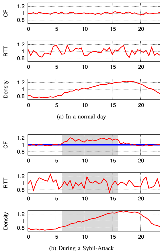
Fig. 8: Evolution of three system metrics in a day, from top Correction Factor, RTT, and node density. Values have been normalized to the average value over that day.
