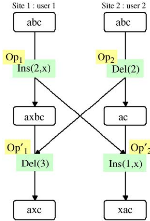
Fig. 7. Scenario violating CP1.
