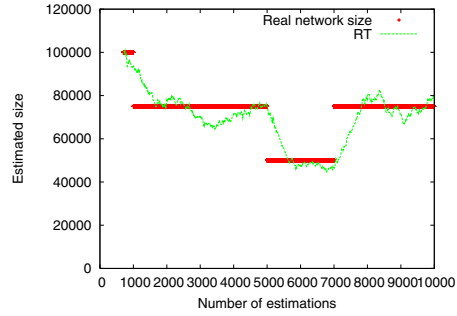
Figure 1: Random Tour with sliding window (last 700) under catastrophic failures; 100,000 nodes at start, -25,000 nodes at runs 1000 and 5000, +25,000 nodes at run 7000.
