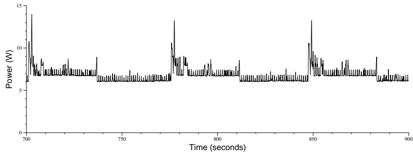
This figure shows how PowerPoint power usage varies over time with a specified autosave frequency of one minute. To generate the measurements, a document was loaded into PowerPoint and modified. The x-axis gives the amount of time that has passed since the modification was performed.
