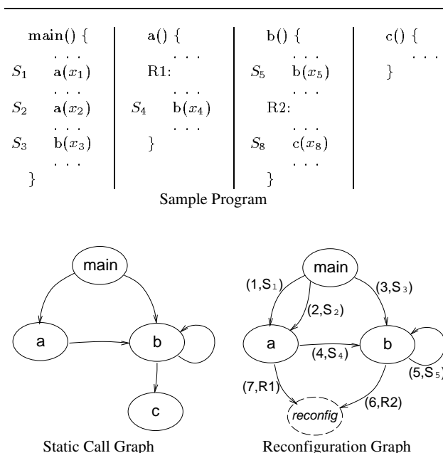
Figure 6: Example of Static Call Graph and Reconfiguration Graph
