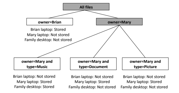
Figure 2: Overlap tree. This figure shows an example overlap tree, constructed from a three-device, three-view scenario: Brian’s files stored on Brian’s laptop, Mary’s files stored on Mary’s laptop, and Mary’s music stored on the Family desktop. Shaded nodes are interior nodes, unshaded nodes are leaf nodes. Each leaf node lists whether this query is stored on each device the household.
