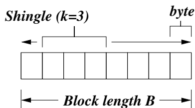
Figure 9. Structure of a disk block (length B ) and shingle ( k contiguous bytes). Here, k = 3 .
