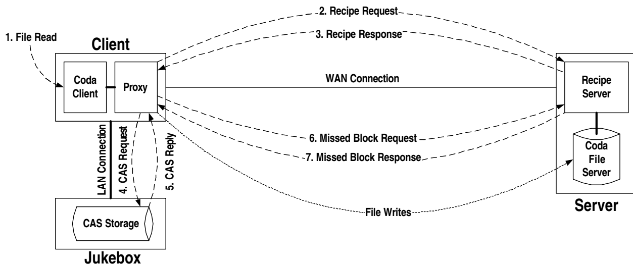
Figure 2. System Diagram
