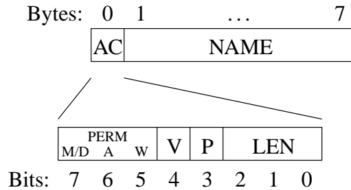
Figure 2. Structure of hierarchically-named capability
