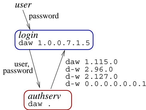
Figure 4. An unprivileged login program acquiring privileges through the authentication server.
