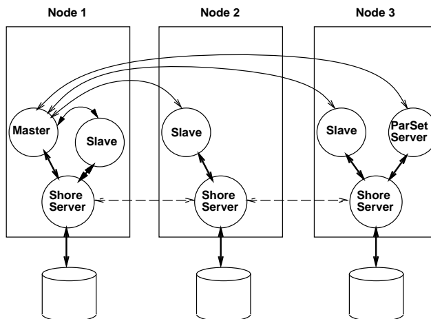
Figure 9: Parallel Shore Architecture
