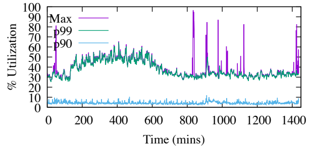
Figure 8: Apply thread utilization across the fleet for a single day, measured over 1-minute periods: for each minute, we show the three clusters with the max / p99 / p90 utilizations. For any given minute, 90% of the clusters are below 10% apply utilization.
