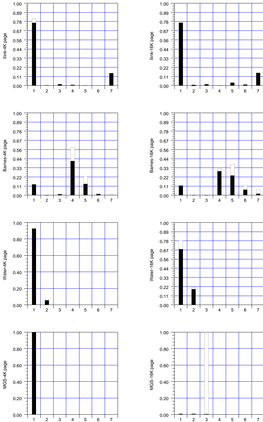
Figure 3: False sharing signature for 4 Kbyte and 16 Kbyte consistency units. On the horizontal axis, the number of requests to concurrent writers as seen at page faults. Each bar represents the frequency of requests of that type. Communication breakdown: black - useful, white - useless
