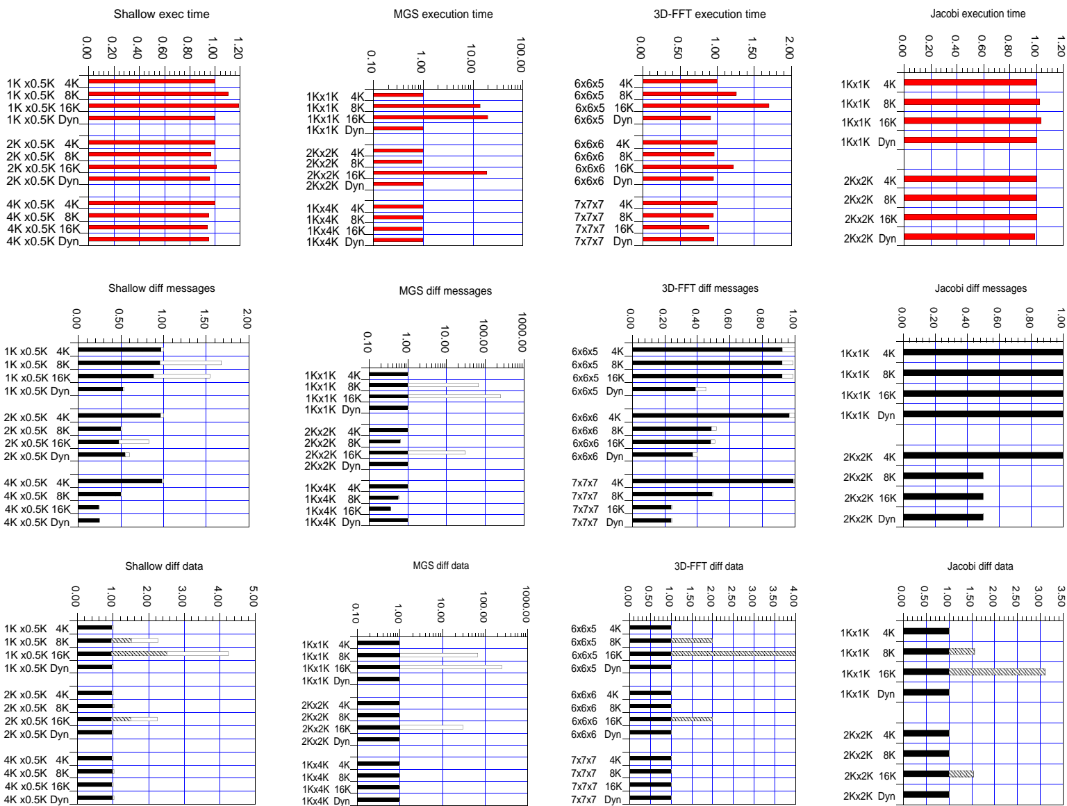
Figure 2: 8-processor execution times, messages, and data, normalized to the corresponding number for 4 Kbytes. Due to the severe degradation, all the statistics in MGS are represented on a logarithmic scale. Communication breakdown: black - useful, white - useless, striped - piggybacked useless data
